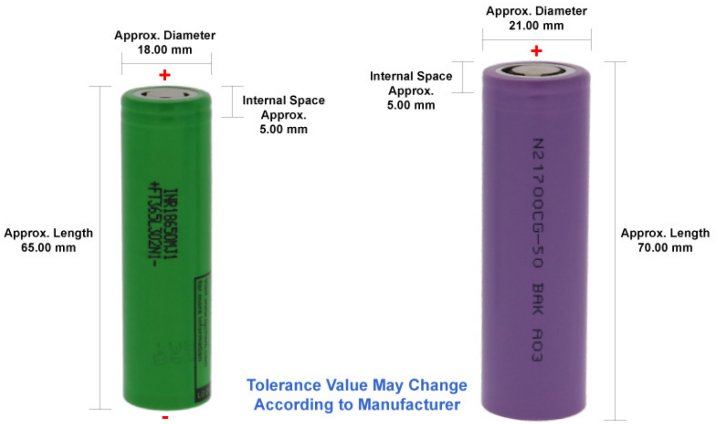
Figure 2: Dimensional characteristics of the 18650 and 21700 cell models.
